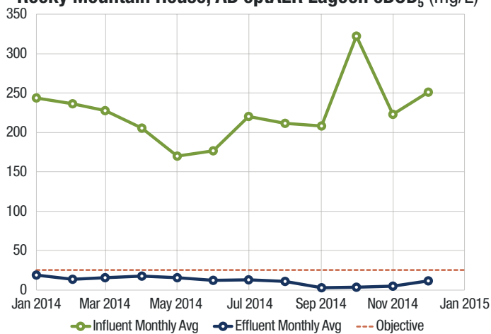
Rocky Mountain House, AB optAER Lagoon cBOD 5 (mg/L)
