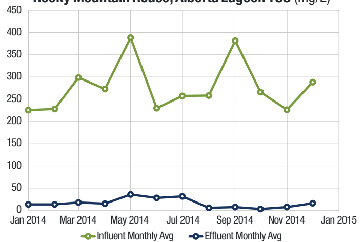
Rocky Mountain House, Alberta Lagoon TSS (mg/L)
