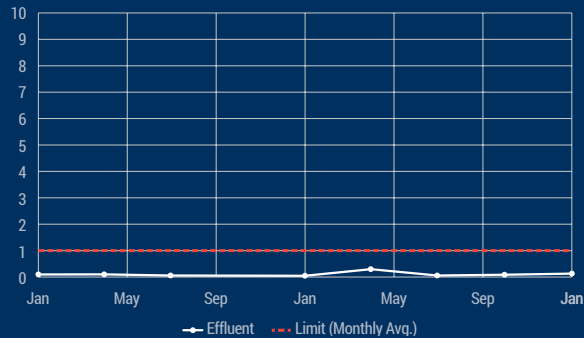
Arizona BioPorts IFAS Total Ammonia-Nitrogen (Daily Max mg/L)
