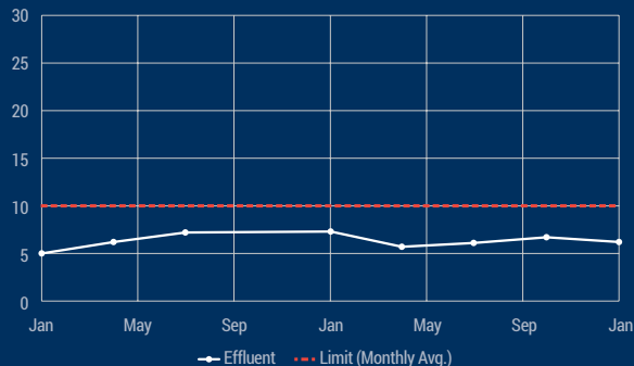
Arizona BioPorts IFAS NO 2 - & NO 3 - (Daily Max mg/L)
